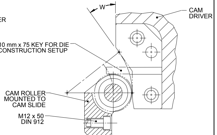
EXAMPLE WITH VERTICAL MOUNT ROLLER
